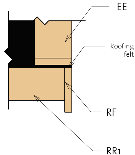
③ Roof Reinforcement
